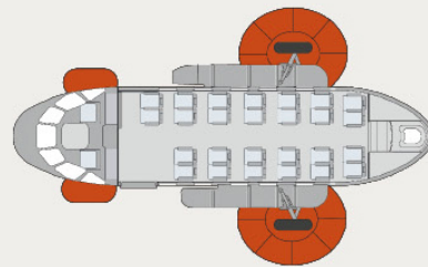
Layout of emergency exits
